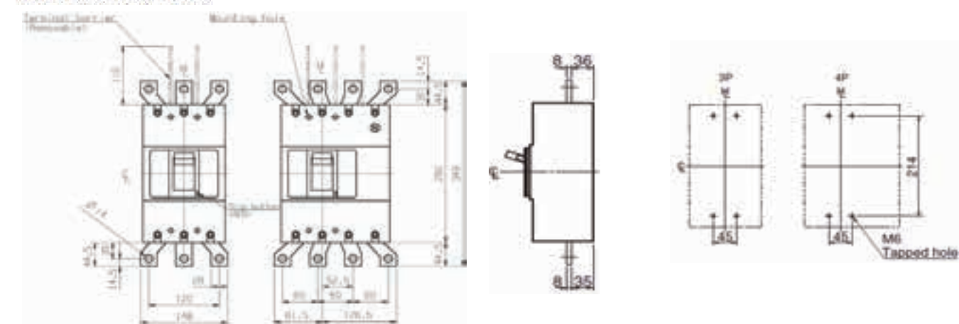
Drilling plan (front view)
